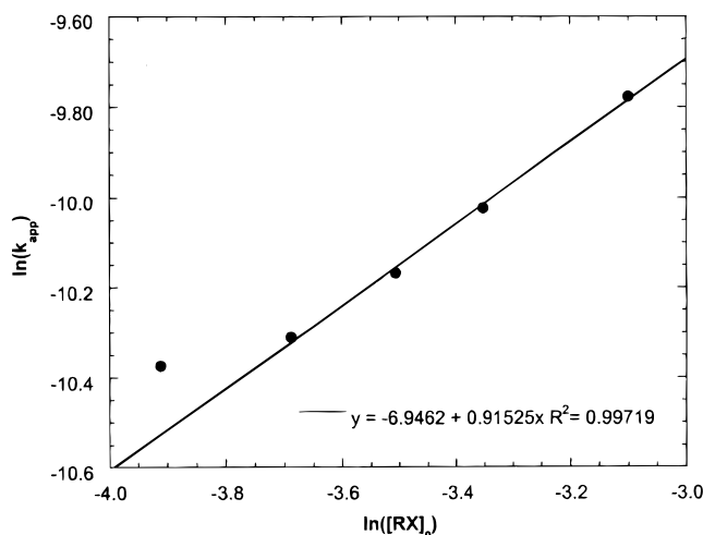
Figure 9. Plots of \ln(k_{app}) as a function of \ln([RX]_0) for simulations of styrene ATRP for limited Cu^I X and Cu^{II} X_2 solubilities ( [Cu^I X]_{max} = 20 mM, [Cu^{II} X_2]_{max} = 1.0 mM; k_{therm} = 0 ). Curve fit through data points for the four highest [RX]_0 used only.
